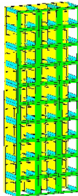
Figure 5 Backing Structure of one Reflector Segment of the CCR 120/100 Reflectors
