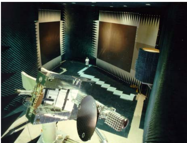
Figure 4 CCR 75/60 with INTELSAT VIII Multi-Feed, Reflector and Mockup Structure
