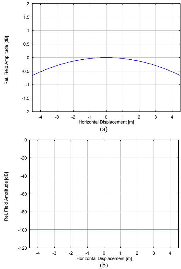
Figure 7 Co- (a) and Cross- (b) Polar Plane Wave Field in the Quiet Zone resulting only from the Feed and Reflectors (without Distortions of the Reflector Rims applied); Minimum Signal Level set to - 100 dB
