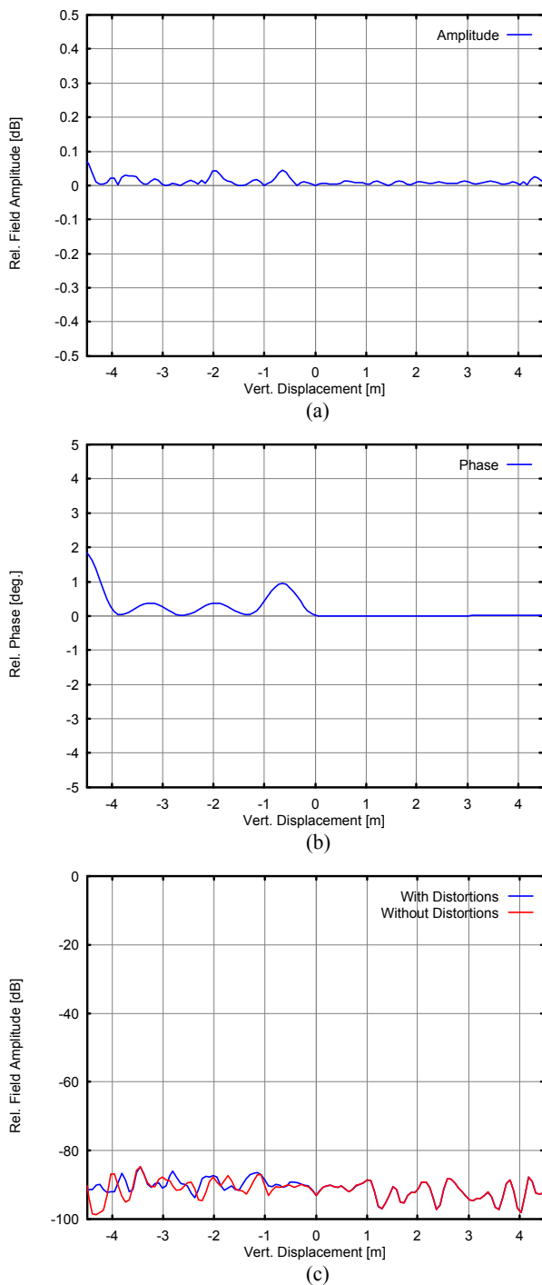
Figure 8 Additional Distortions of Plane Wave Field in the Quiet Zone according to 5 \mu\text{m} Reflector Surface Distortions at Sub- and Main Reflector of CCR 120/100 at a Frequency of 100 GHz:
